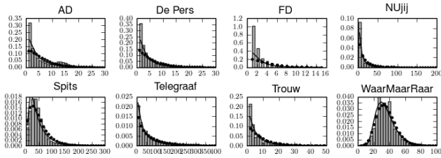
Figure 1: Modeling comment distribution per source using the continuous log-normal distribution (black line). The grey bars represent the observed data. y -axis stands for probability density, and x -axis stands for number of comments (binned).
